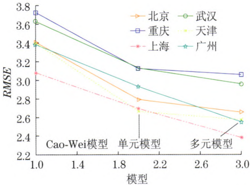
图 3 多元模型与其它模型的 RMSE 比较 Fig.3 RMSE comparison between the multivariate model and other models
